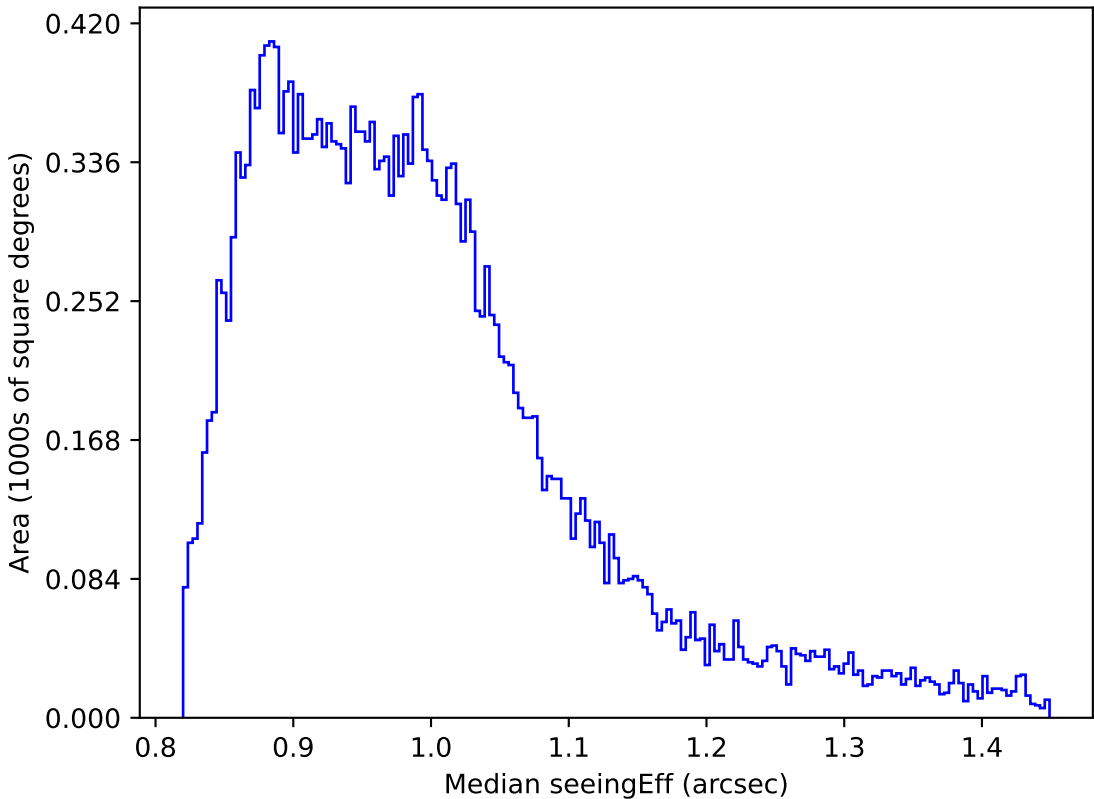
too_elab_r256_d2_griz_v3.4_10yrs Yr 1 all bands: Median seeingEff
