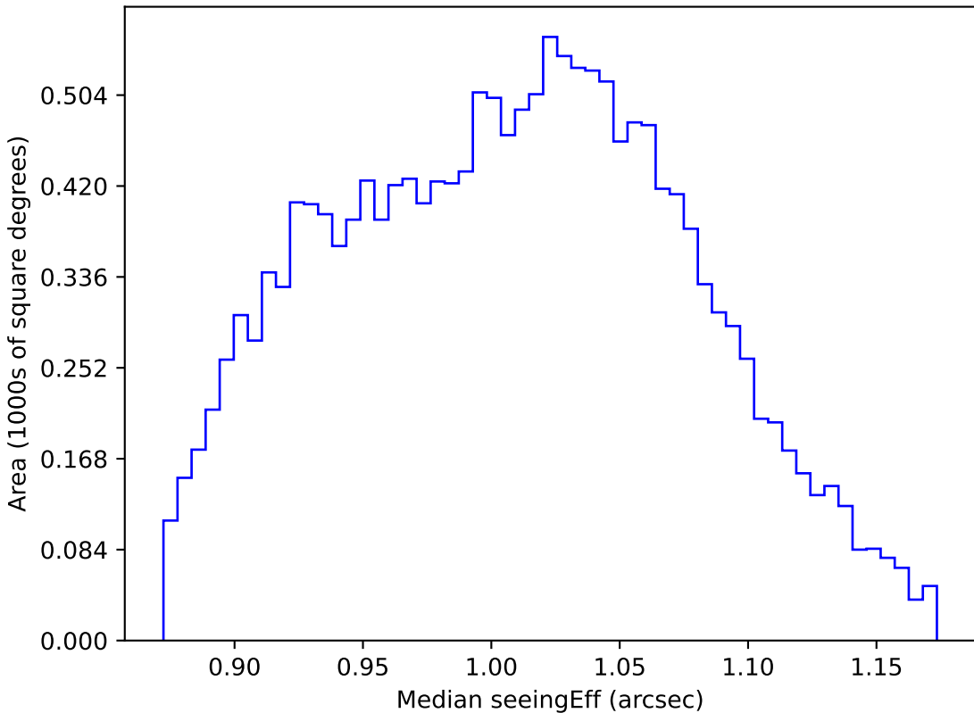
too_elab_r256_d2_griz_v3.4_10yrs WFD z band: Median seeingEff
