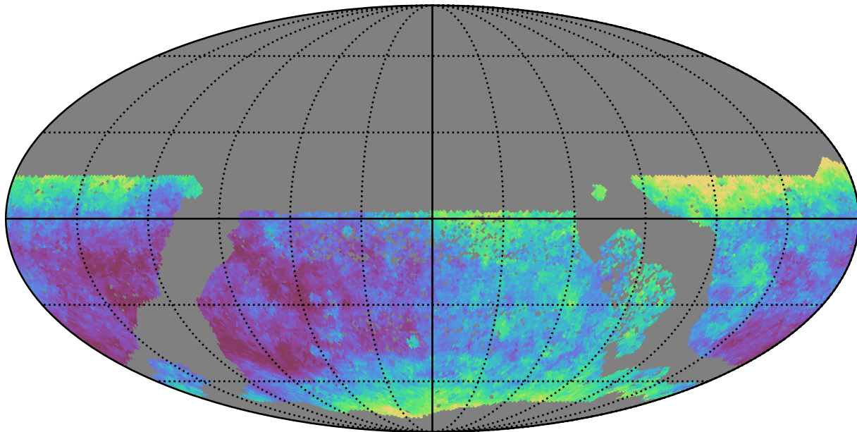
too_elab_r256_d2_griz_v3.4_10yrs WFD y band: Median seeingEff
