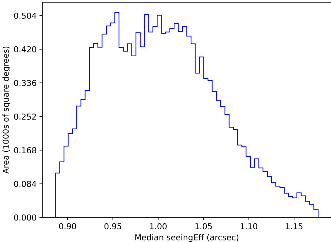
too_elab_r256_d2_griz_v3.4_10yrs WFD y band: Median seeingEff
