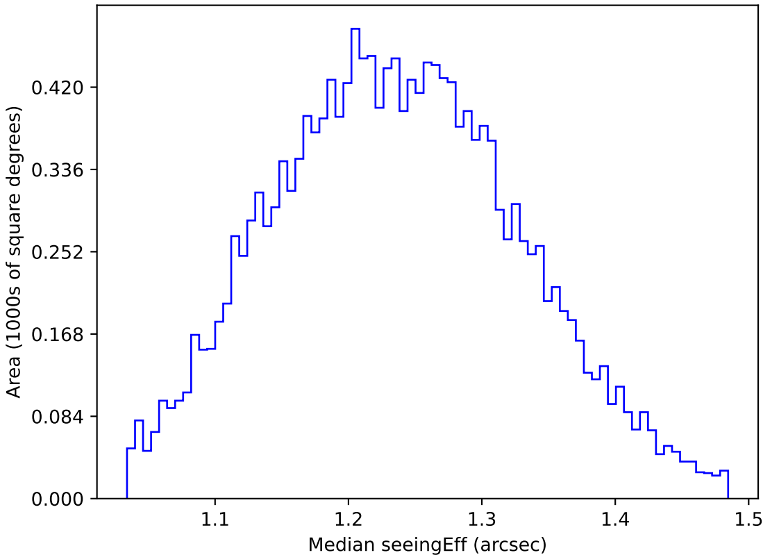
too_elab_r256_d2_griz_v3.4_10yrs WFD u band: Median seeingEff
