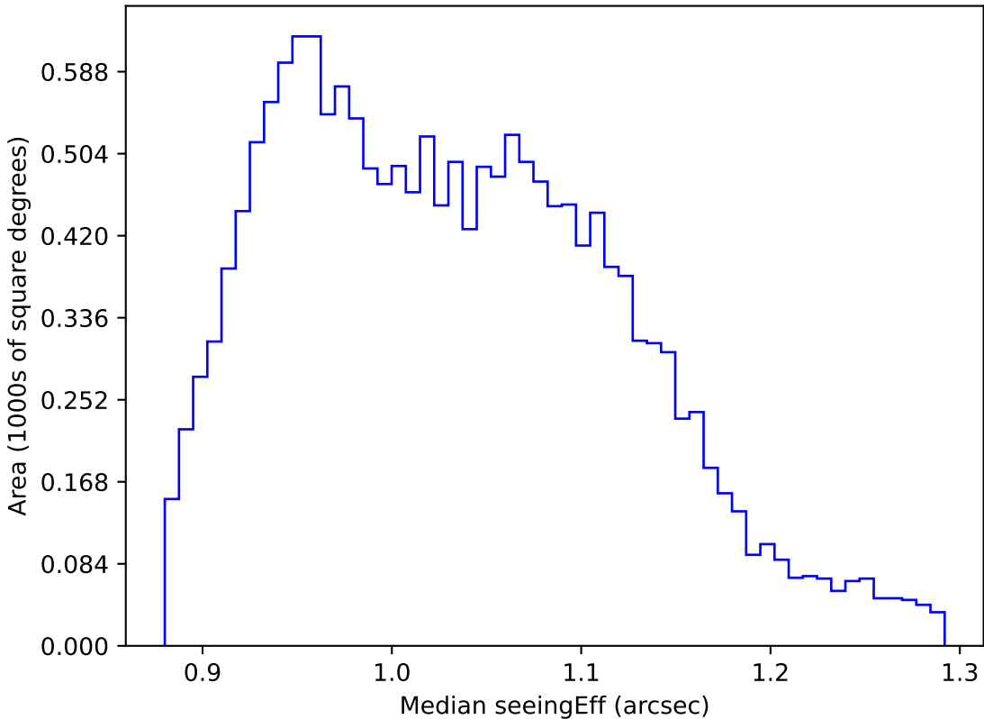
too_elab_r256_d2_griz_v3.4_10yrs WFD r band: Median seeingEff
