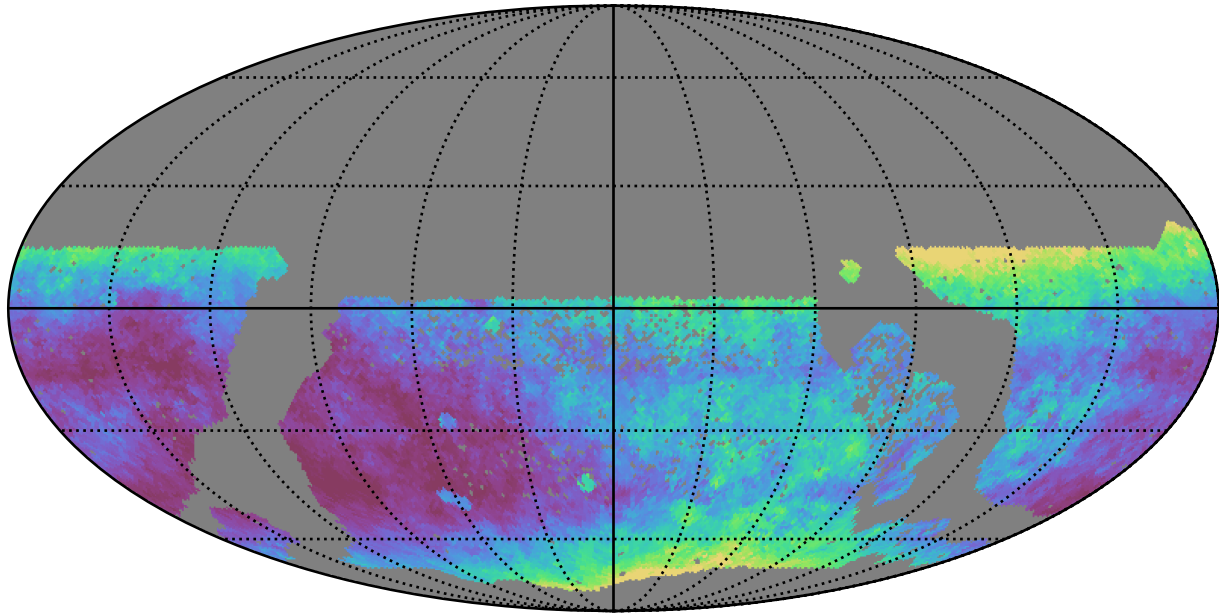
too_elab_r256_d2_griz_v3.4_10yrs WFD i band: Median seeingEff
