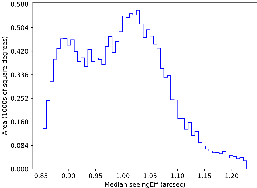
too_elab_r256_d2_griz_v3.4_10yrs WFD i band: Median seeingEff
