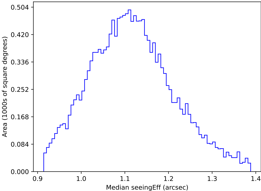
too_elab_r256_d2_griz_v3.4_10yrs WFD g band: Median seeingEff
