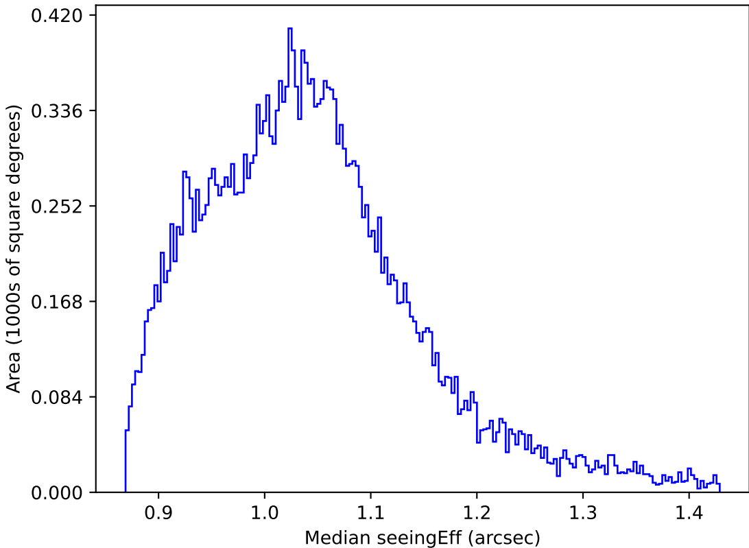
too_elab_r256_d2_griz_v3.4_10yrs All sky z band: Median seeingEff
