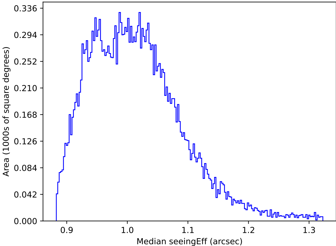
too_elab_r256_d2_griz_v3.4_10yrs All sky y band: Median seeingEff
