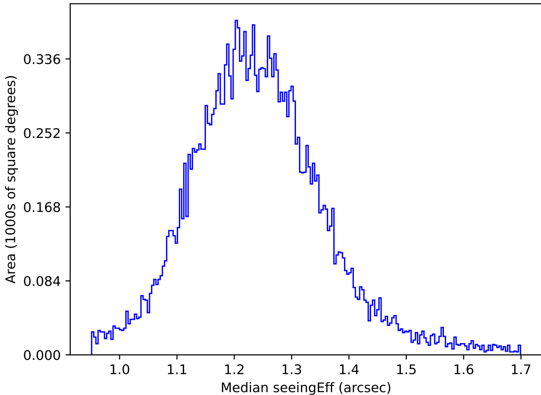
too_elab_r256_d2_griz_v3.4_10yrs All sky u band: Median seeingEff
