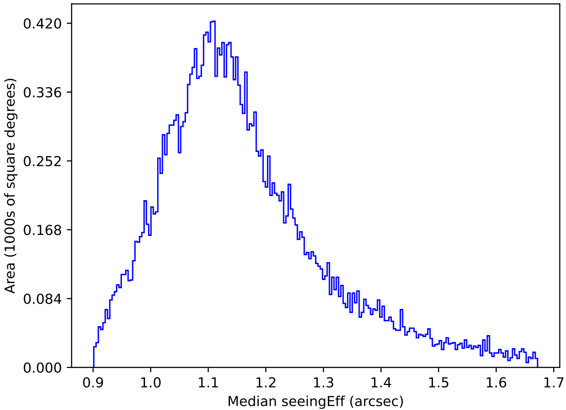
too_elab_r256_d2_griz_v3.4_10yrs All sky g band: Median seeingEff
