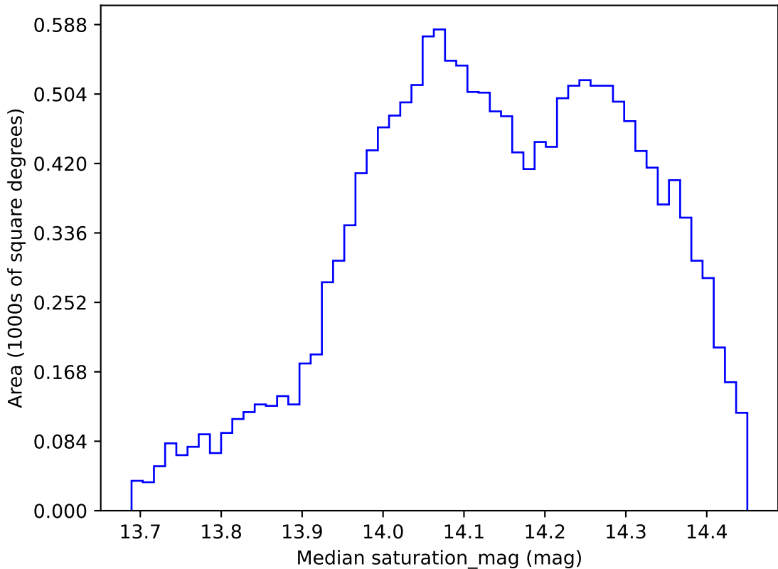
too_elab_r256_d2_griz_v3.4_10yrs WFD all bands: Median saturation_mag
