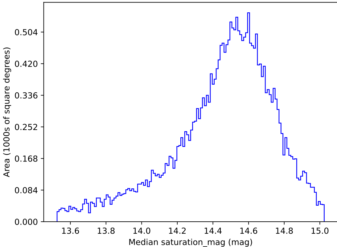
too_elab_r256_d2_griz_v3.4_10yrs All sky g band: Median saturation_mag
