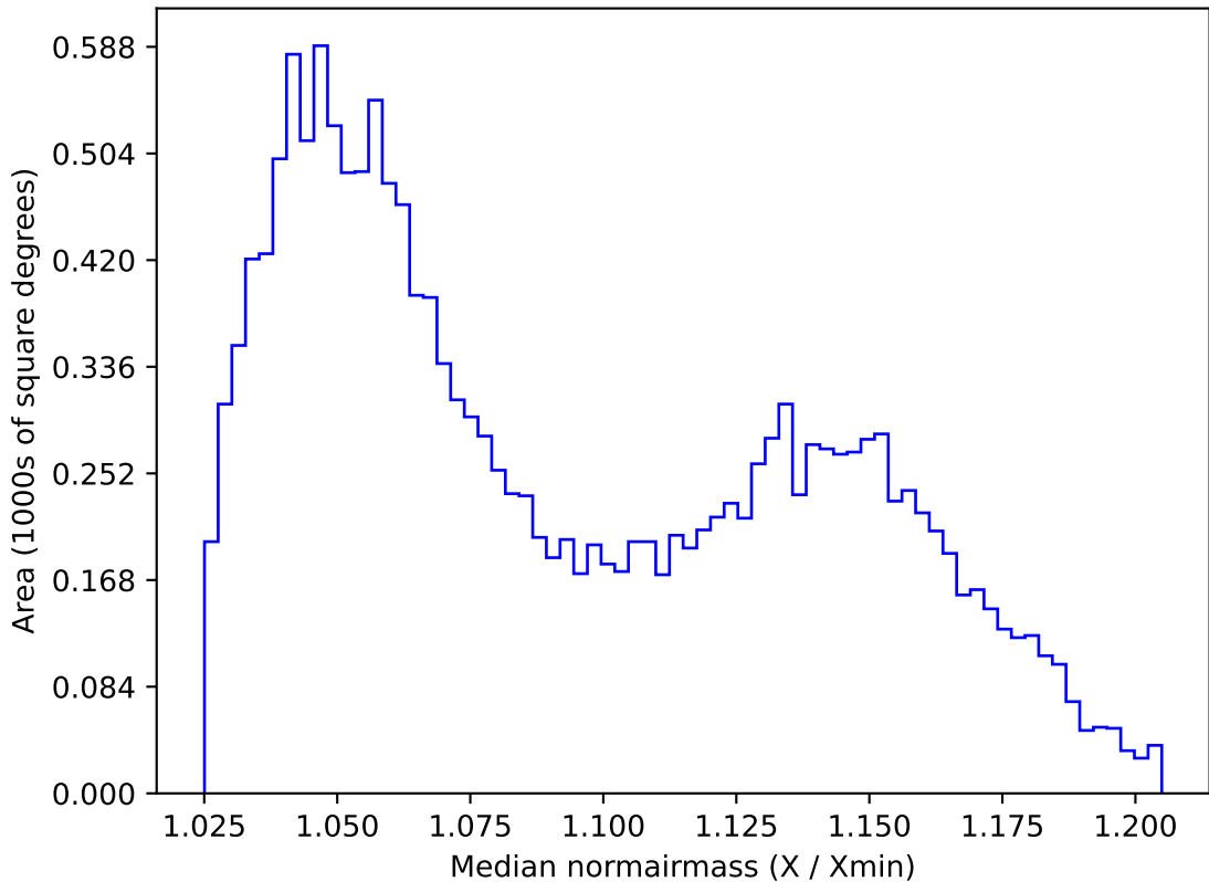
too_elab_r256_d2_griz_v3.4_10yrs WFD z band: Median normairmass
