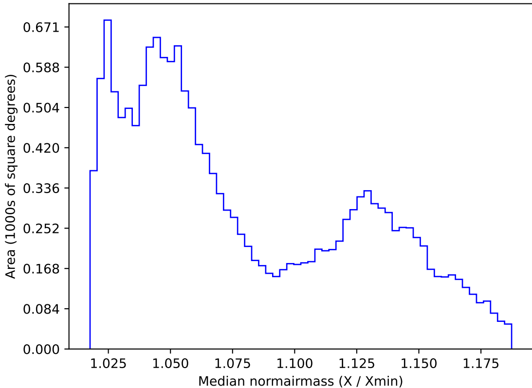
too_elab_r256_d2_griz_v3.4_10yrs WFD r band: Median normairmass
