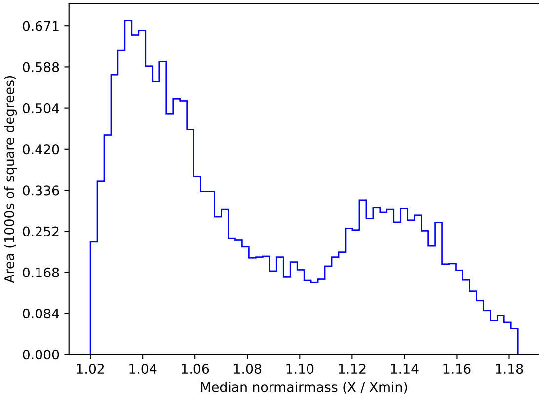
too_elab_r256_d2_griz_v3.4_10yrs WFD i band: Median normairmass
