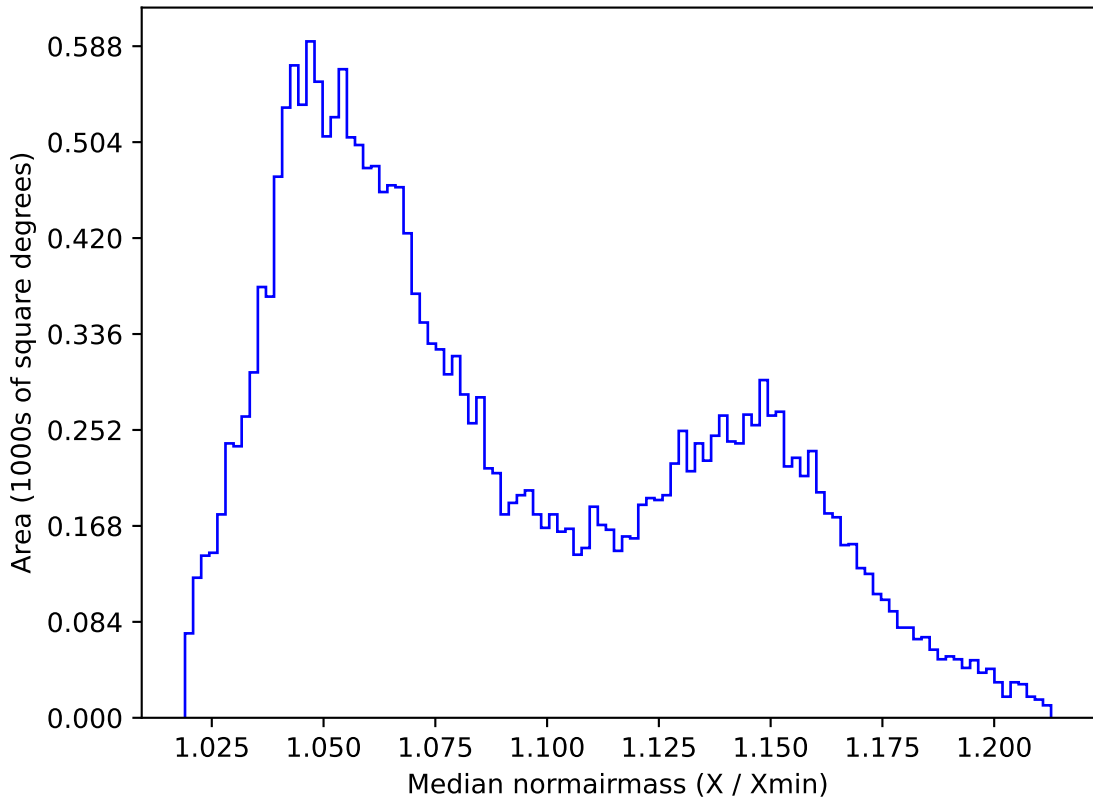
too_elab_r256_d2_griz_v3.4_10yrs All sky y band: Median normairmass
