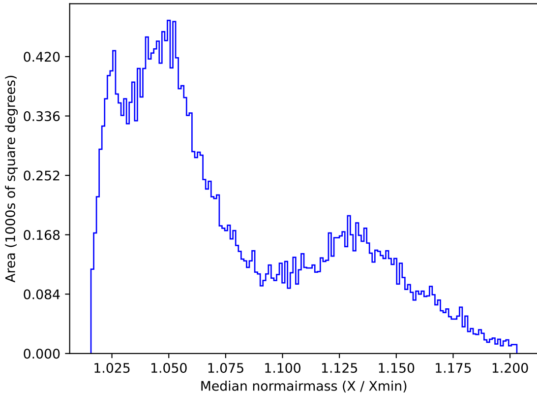
too_elab_r256_d2_griz_v3.4_10yrs All sky r band: Median normairmass
