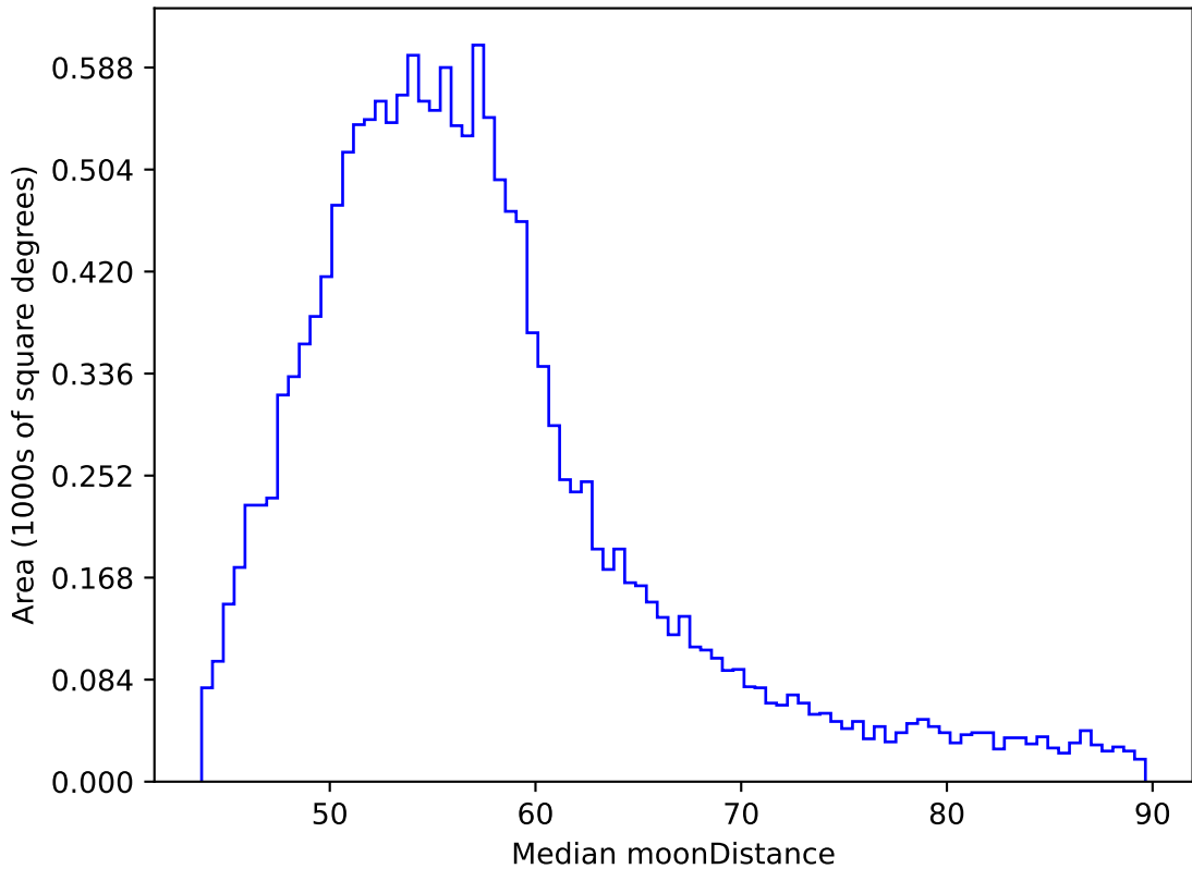
too_elab_r256_d2_griz_v3.4_10yrs WFD y band: Median moonDistance
