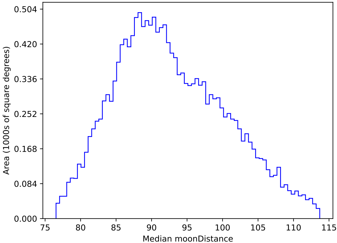
too_elab_r256_d2_griz_v3.4_10yrs WFD i band: Median moonDistance
