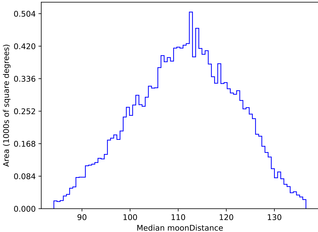
too_elab_r256_d2_griz_v3.4_10yrs WFD g band: Median moonDistance
