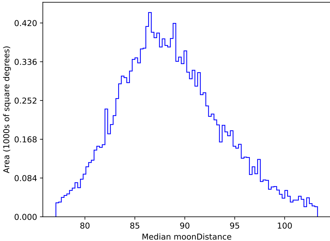
too_elab_r256_d2_griz_v3.4_10yrs WFD all bands: Median moonDistance
