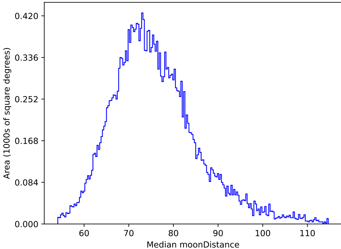
too_elab_r256_d2_griz_v3.4_10yrs All sky z band: Median moonDistance
