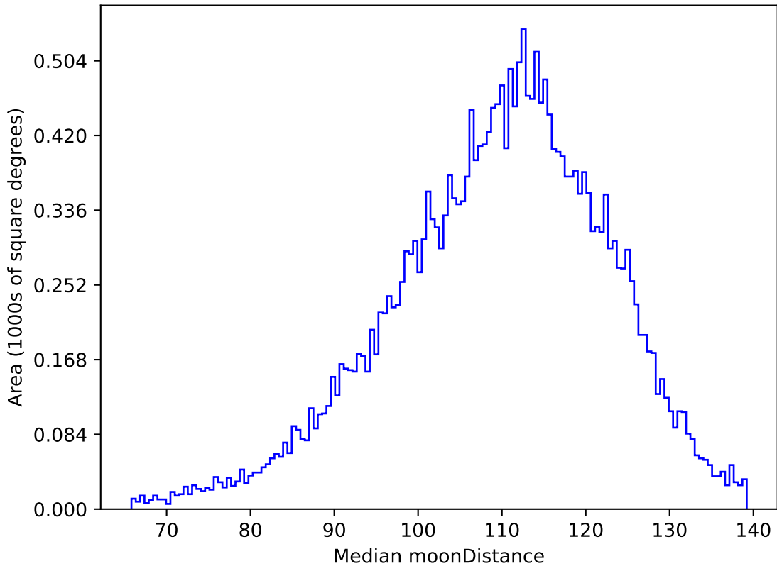
too_elab_r256_d2_griz_v3.4_10yrs All sky g band: Median moonDistance
