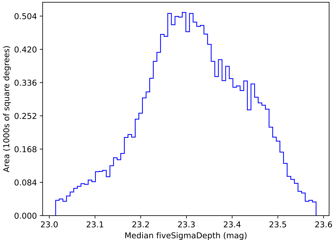
too_elab_r256_d2_griz_v3.4_10yrs WFD all bands: Median fiveSigmaDepth
