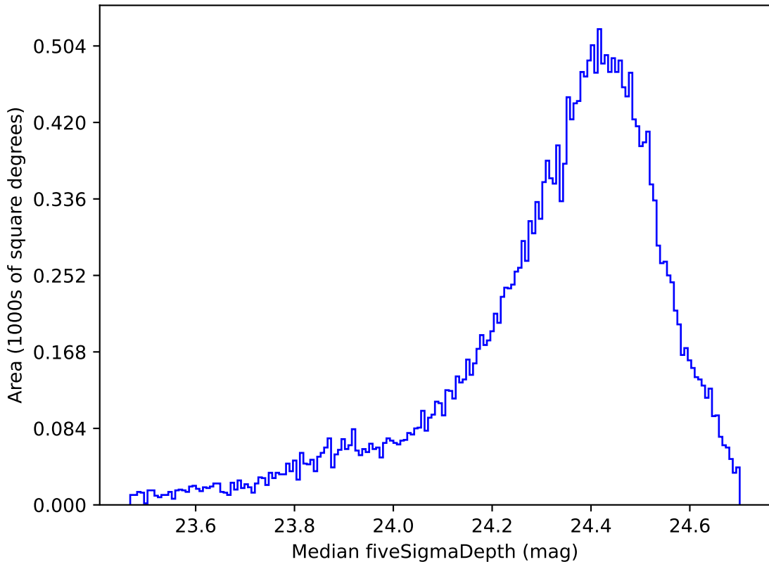
too_elab_r256_d2_griz_v3.4_10yrs All sky g band: Median fiveSigmaDepth
