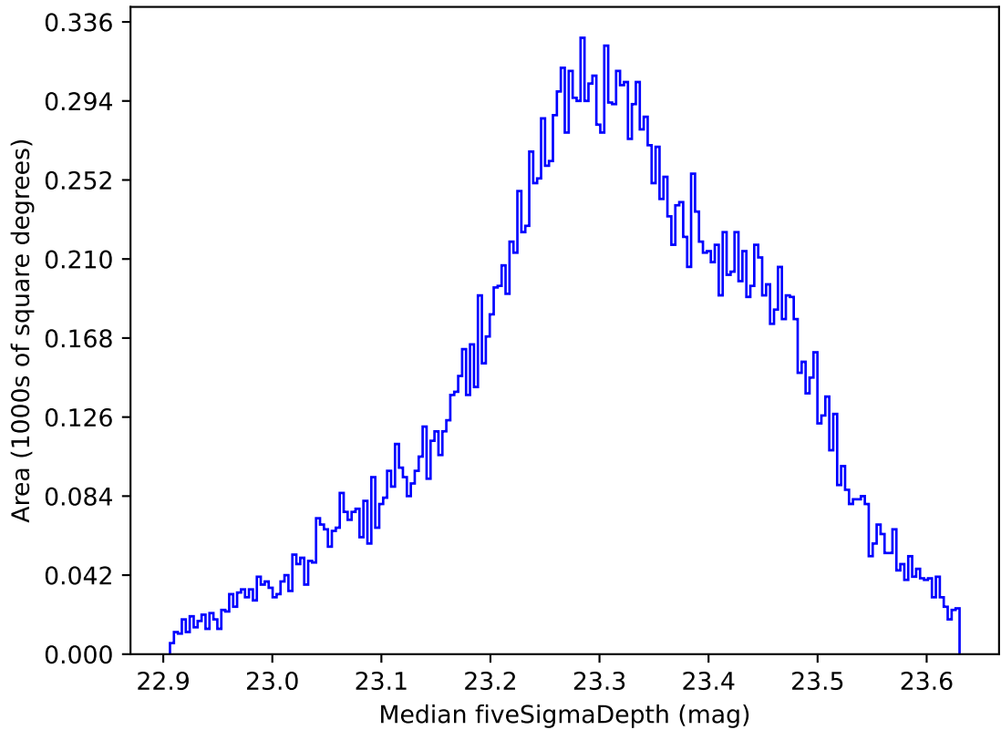
too_elab_r256_d2_griz_v3.4_10yrs All sky all bands: Median fiveSigmaDepth
