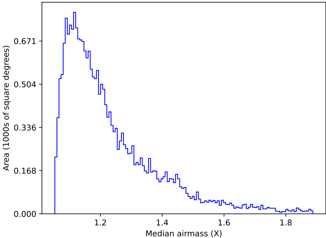
too_elab_r256_d2_griz_v3.4_10yrs Yr 1 u band: Median airmass
