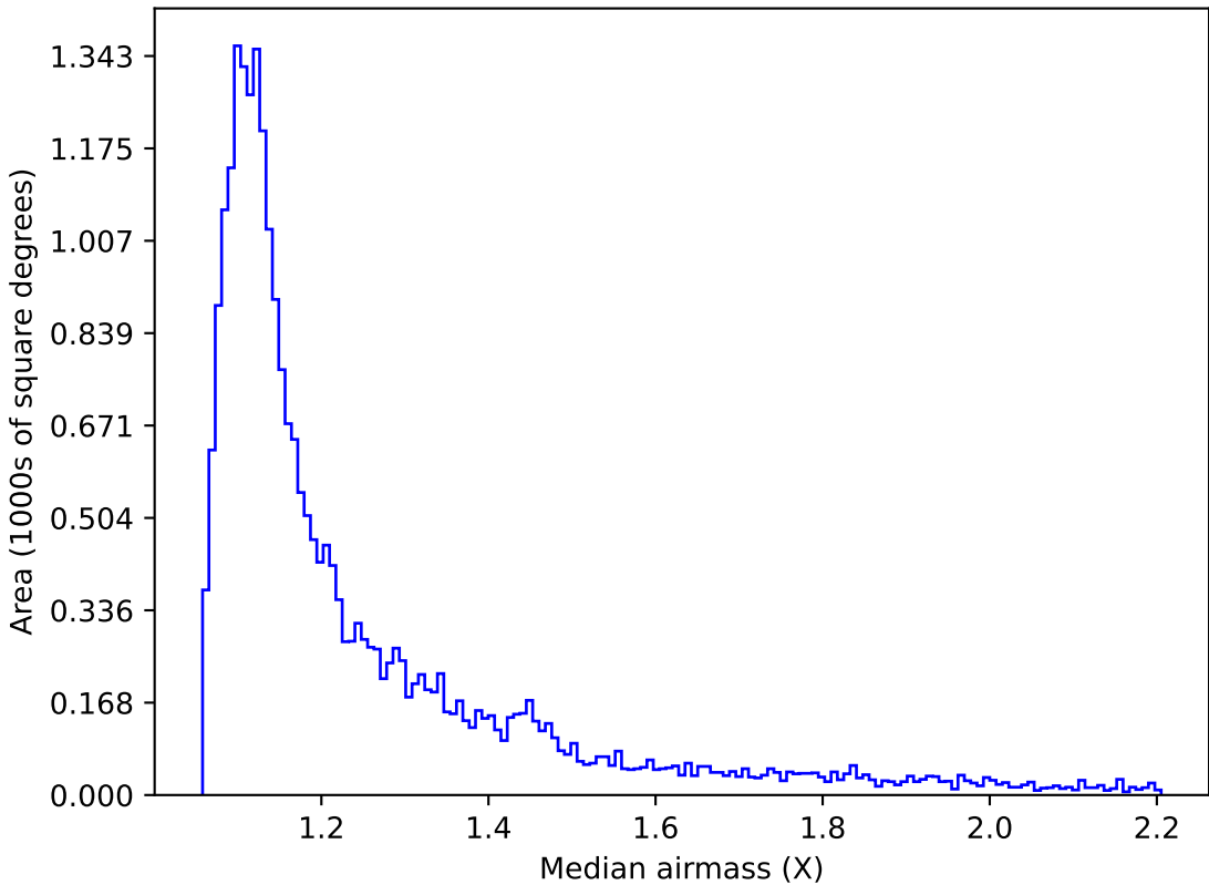
too_elab_r256_d2_griz_v3.4_10yrs Yr 1 i band: Median airmass
