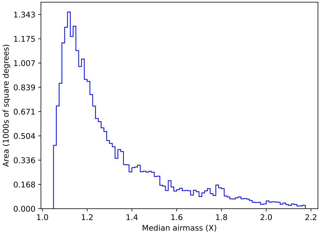
too_elab_r256_d2_griz_v3.4_10yrs Yr 1 g band: Median airmass
