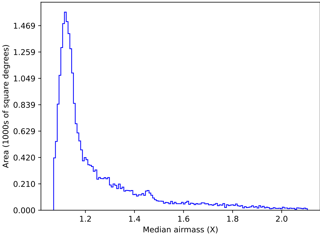
too_elab_r256_d2_griz_v3.4_10yrs Yr 1 all bands: Median airmass
