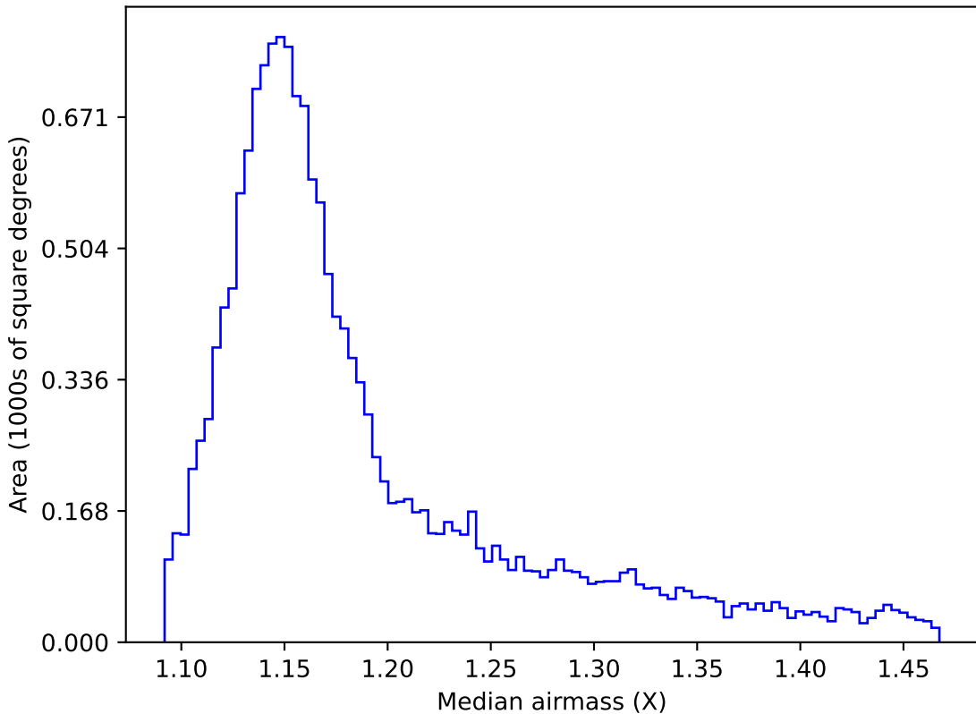
too_elab_r256_d2_griz_v3.4_10yrs WFD z band: Median airmass
