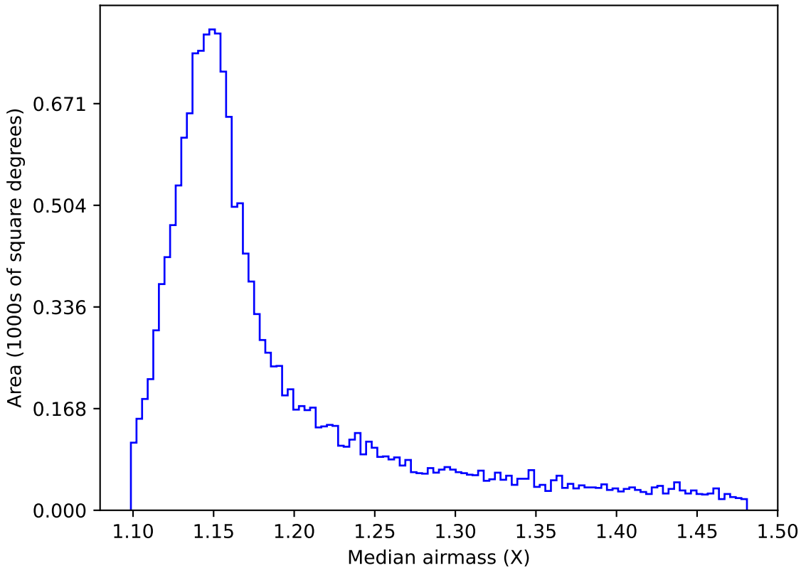
too_elab_r256_d2_griz_v3.4_10yrs WFD y band: Median airmass
