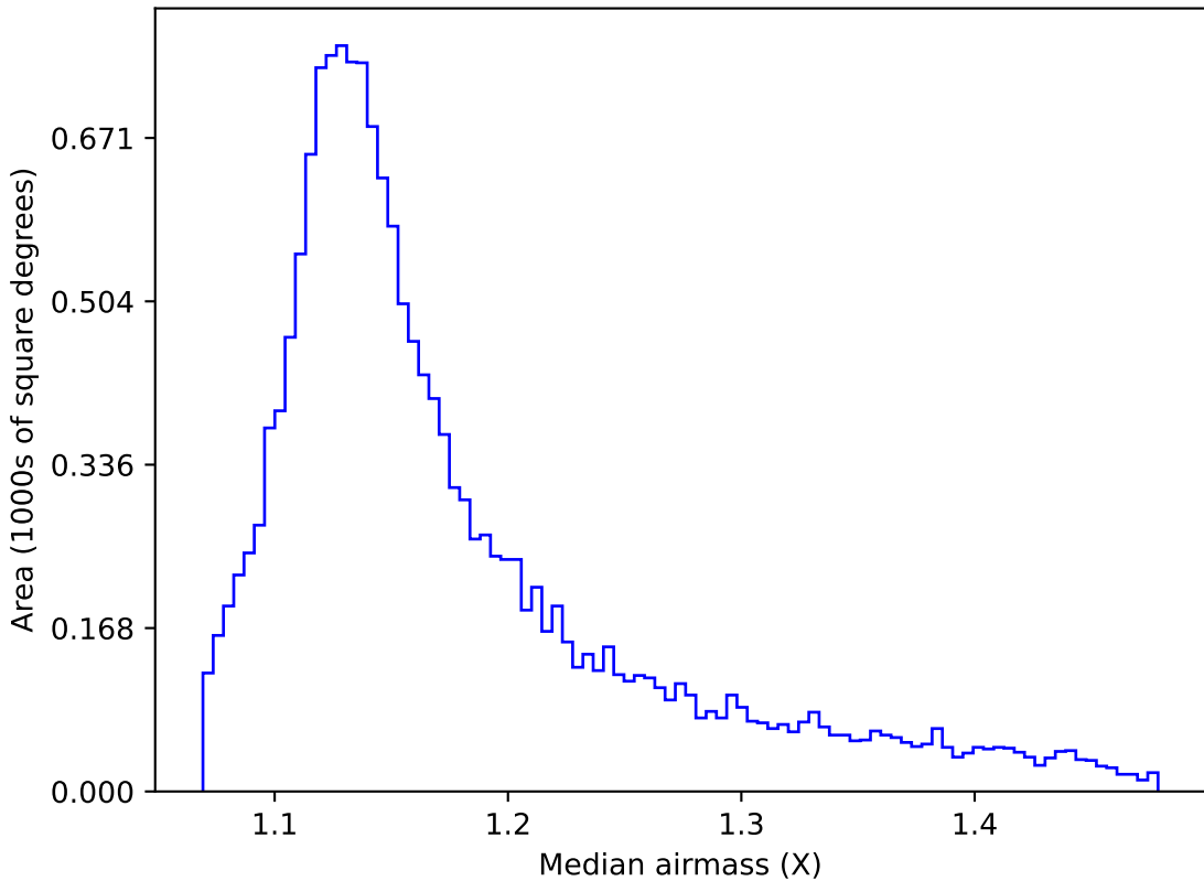
too_elab_r256_d2_griz_v3.4_10yrs WFD u band: Median airmass
