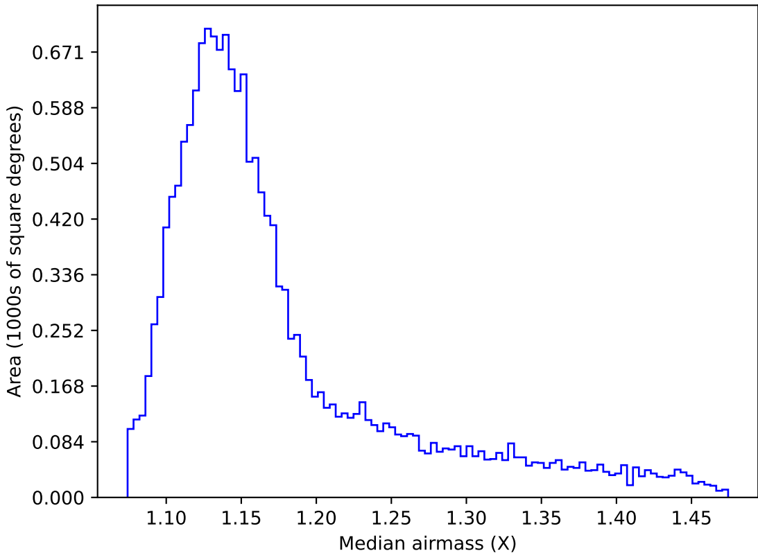
too_elab_r256_d2_griz_v3.4_10yrs WFD r band: Median airmass
