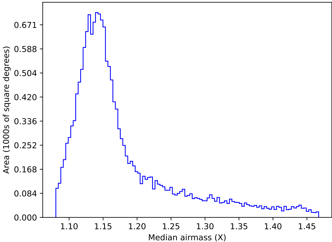
too_elab_r256_d2_griz_v3.4_10yrs WFD i band: Median airmass
