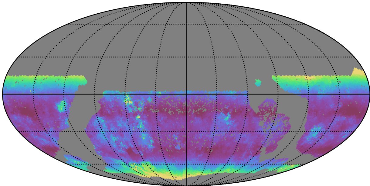
too_elab_r256_d2_griz_v3.4_10yrs WFD g band: Median airmass
