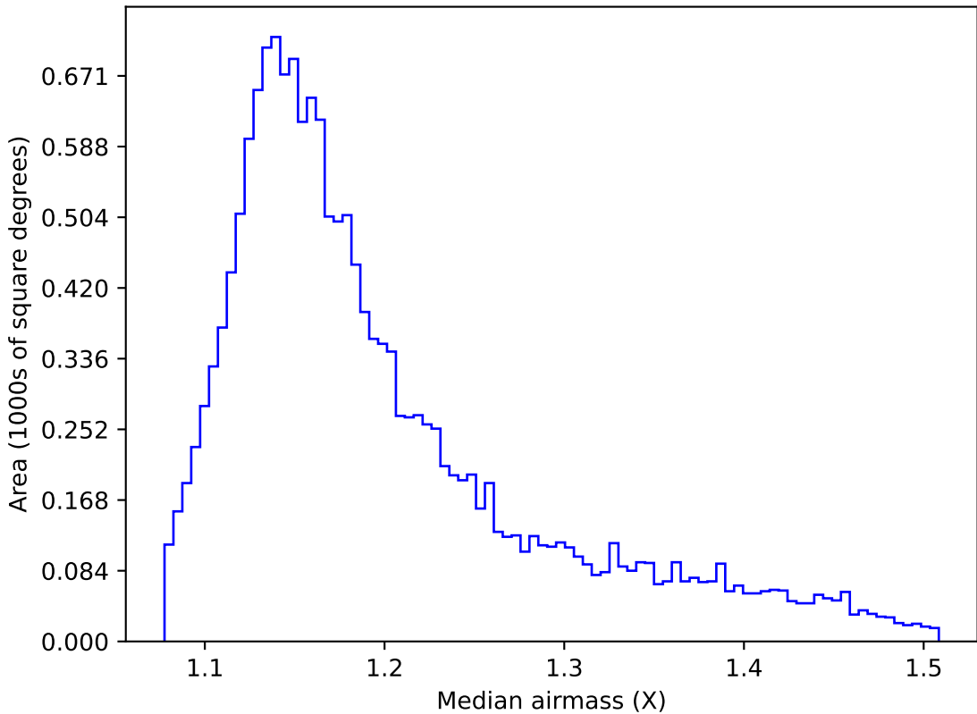
too_elab_r256_d2_griz_v3.4_10yrs WFD g band: Median airmass
