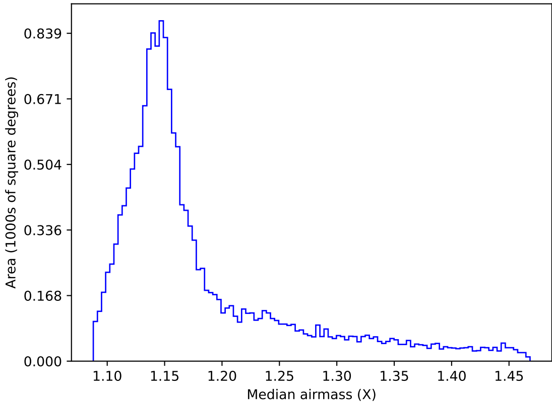
too_elab_r256_d2_griz_v3.4_10yrs WFD all bands: Median airmass
