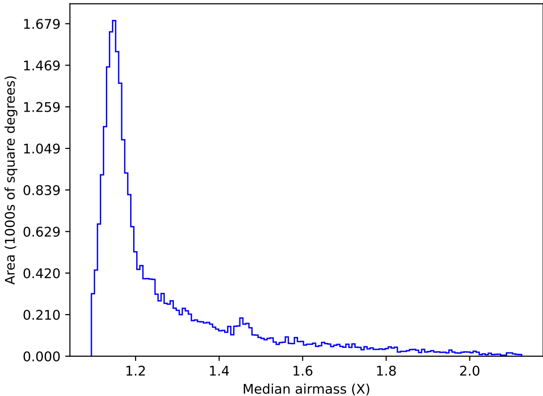
too_elab_r256_d2_griz_v3.4_10yrs All sky z band: Median airmass
