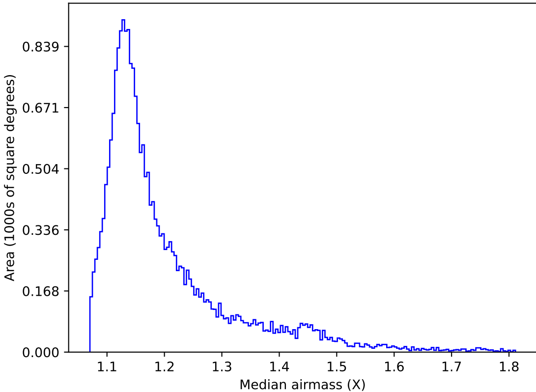
too_elab_r256_d2_griz_v3.4_10yrs All sky u band: Median airmass
