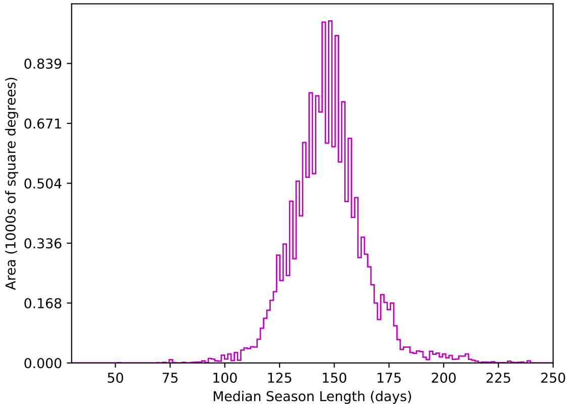
too_elab_r256_d2_griz_v3.4_10yrs WFD z band: Median Season Length
