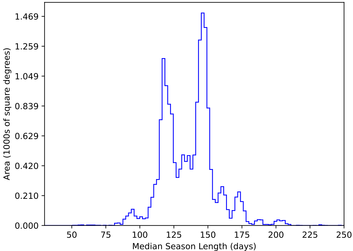
too_elab_r256_d2_griz_v3.4_10yrs WFD y band: Median Season Length
