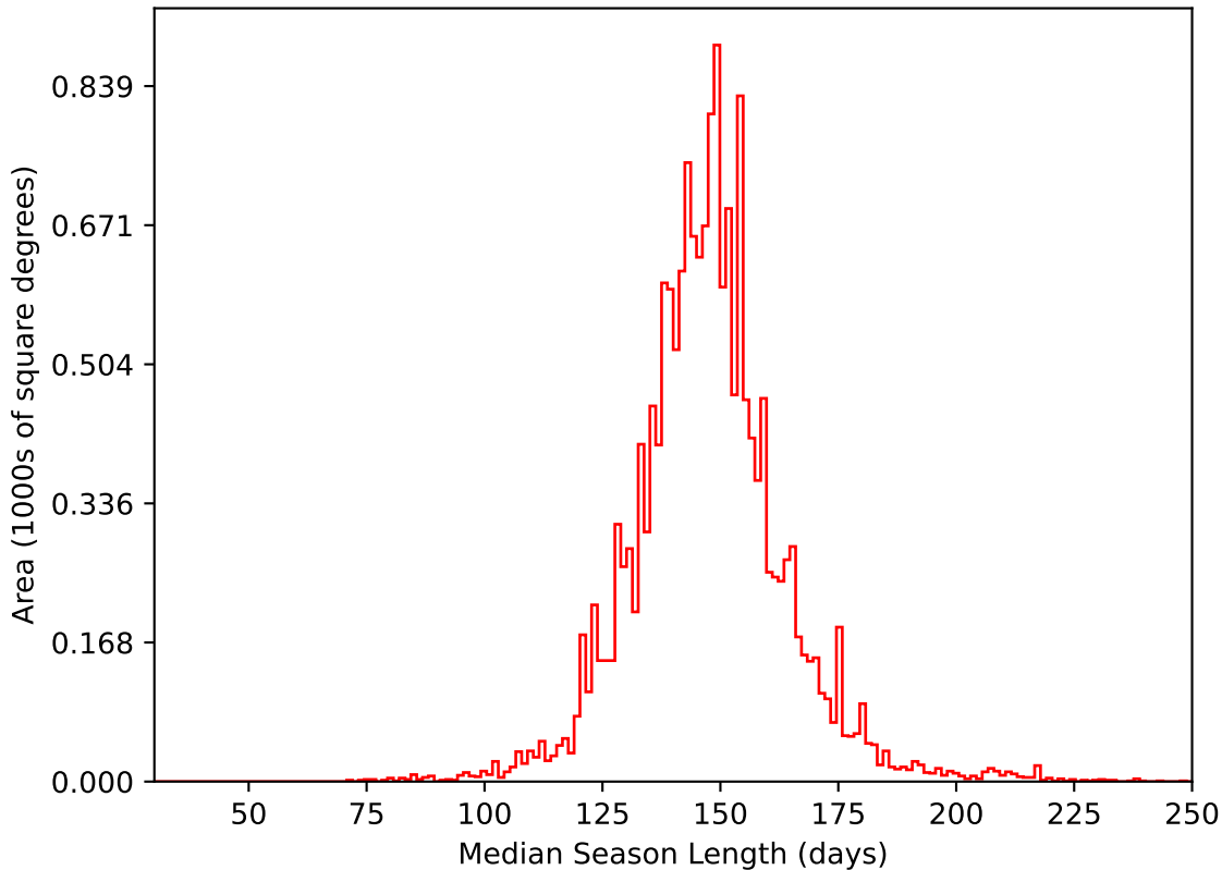
too_elab_r256_d2_griz_v3.4_10yrs WFD i band: Median Season Length
