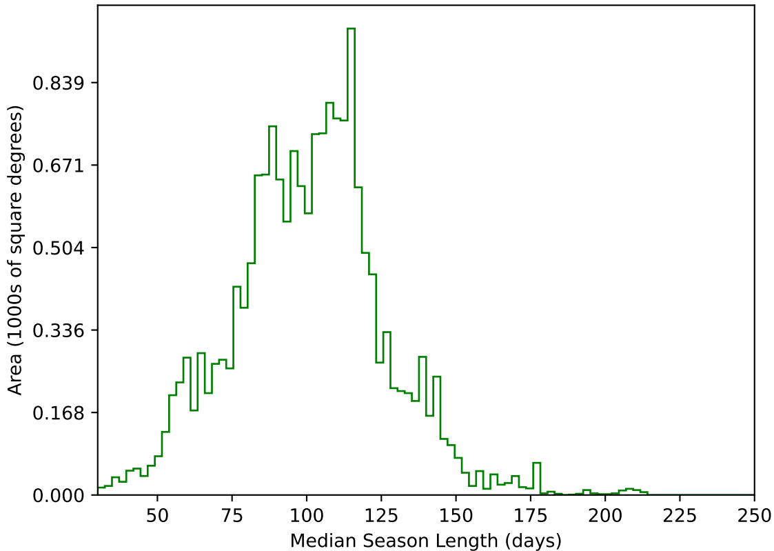
too_elab_r256_d2_griz_v3.4_10yrs WFD g band: Median Season Length
