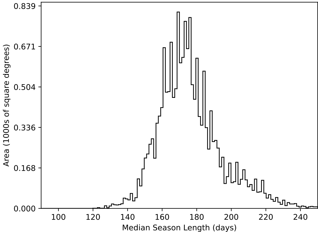
too_elab_r256_d2_griz_v3.4_10yrs WFD all bands: Median Season Length
