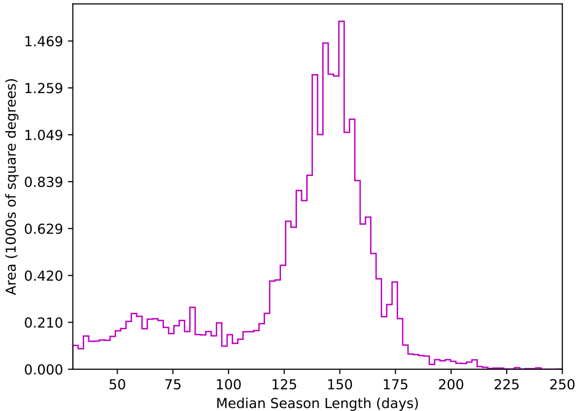
too_elab_r256_d2_griz_v3.4_10yrs All sky z band: Median Season Length
