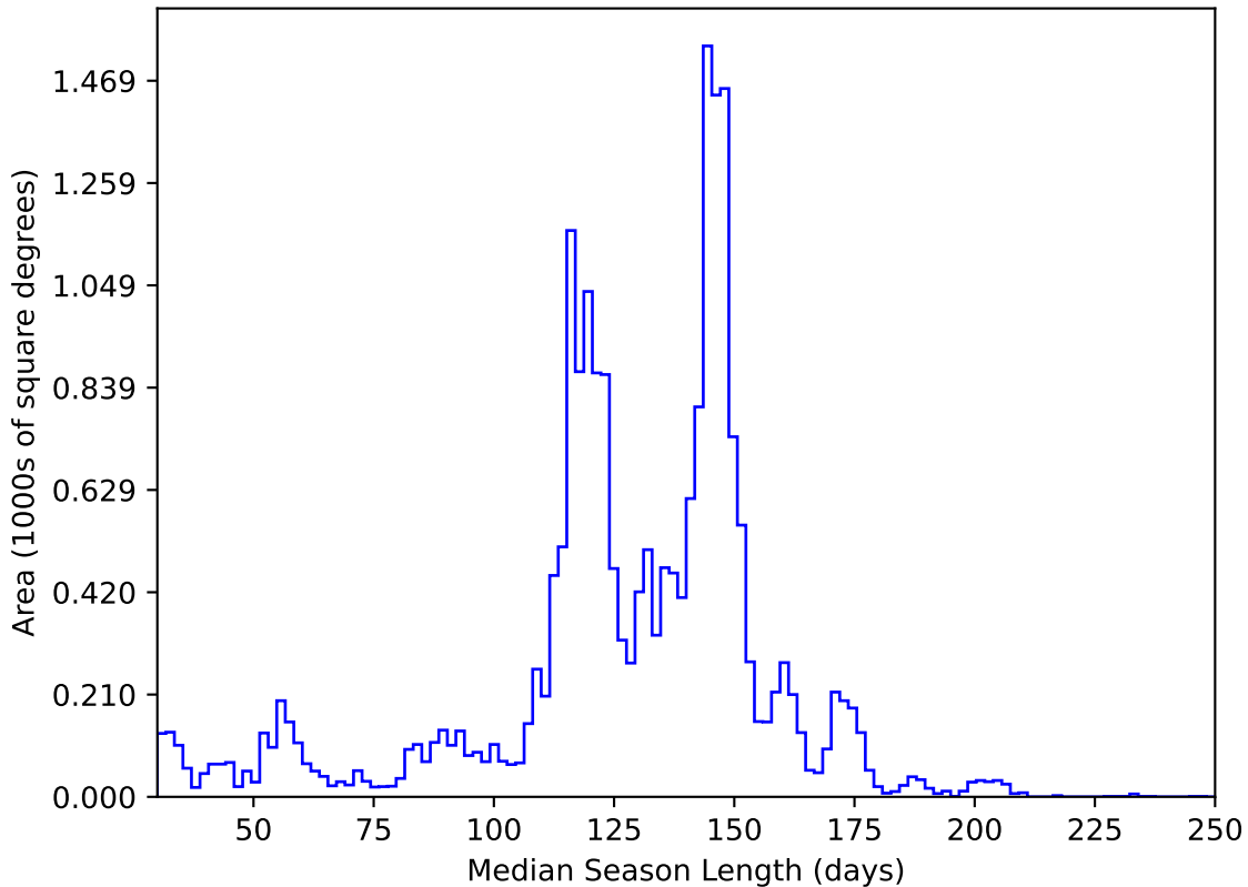
too_elab_r256_d2_griz_v3.4_10yrs All sky y band: Median Season Length
